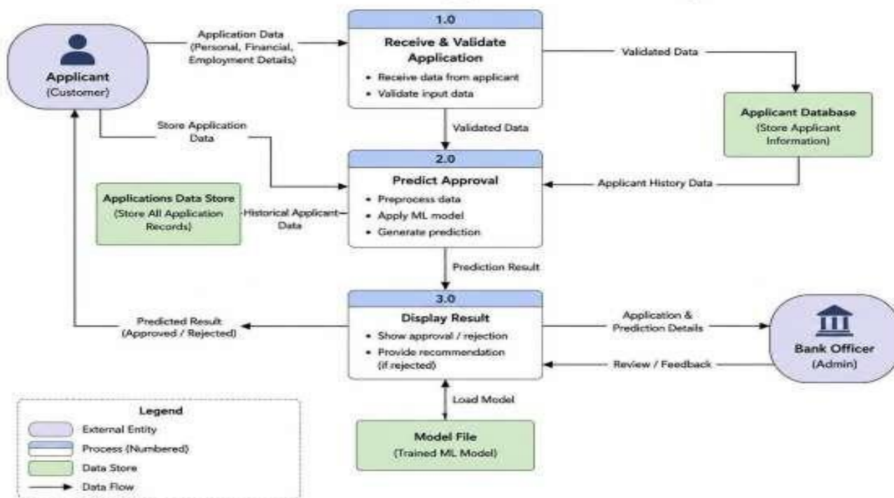
DFD – Credit Card Approval Prediction System
